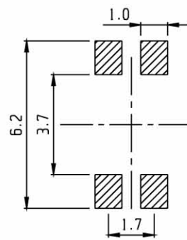
PCB LAYOUT
