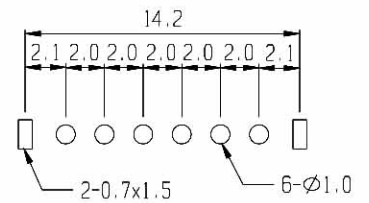
PCB LAYOUT
