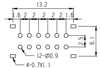
PCB LAYOUT
