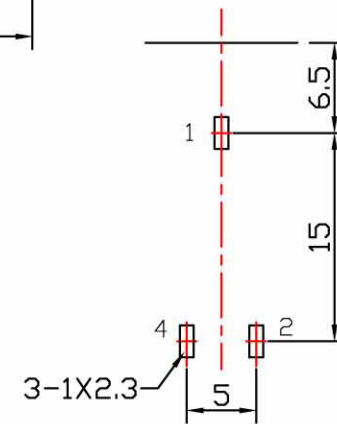
PCB MOUNTING HOLES (VIEWED FROM COPPER SIDE)
