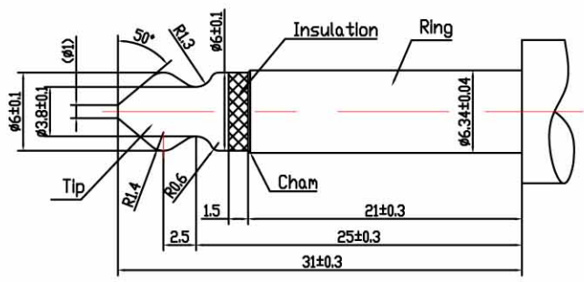
MONO PLUG
