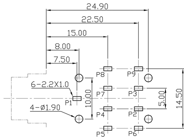
RECOMMENDED PCB LAYOUT T=1.6mm TOP VIEW TOLERANCE: ±0.05
