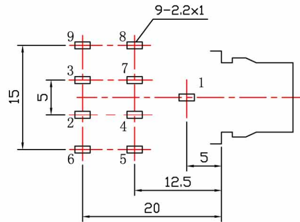
PCB MOUNTING HOLES (TOLERANCE: \pm 0.1 ) (BOTTOM VIEW)
