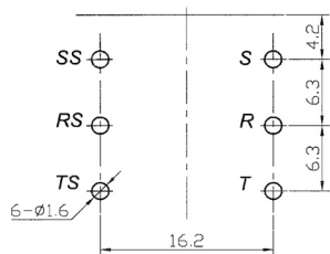
PCB MOUNTING HOLES (VIEWED FROM COPPER SIDE)
