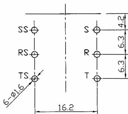
PCB MOUNTING HOLES (VIEWED FROM COPPER SIDE)
