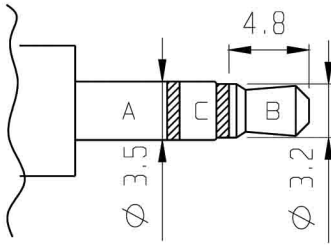
MATING PLUG
