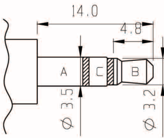
MATING PLUG
