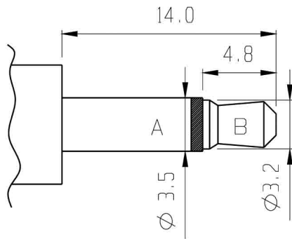
MATING PLUG
