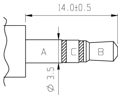
MATING PLUG
