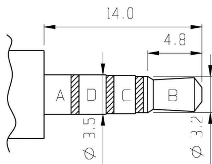
MATING PLUG
