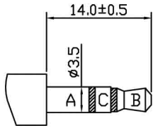
MATING PLUG
