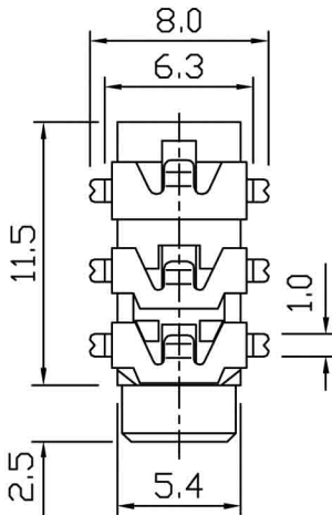
MATING PLUG
