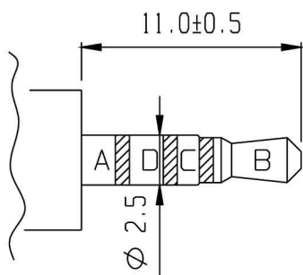
MATING PLUG
