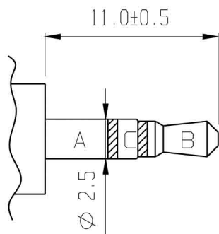
MATING PLUG
