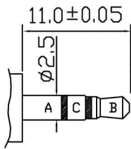
MATING PLUG
