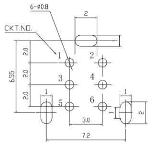
PCB BOARD LAYOUT
