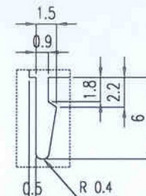
DETAIL "X"
