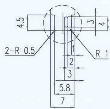
DETAIL "X"
