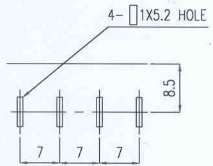
PCB-MTG
