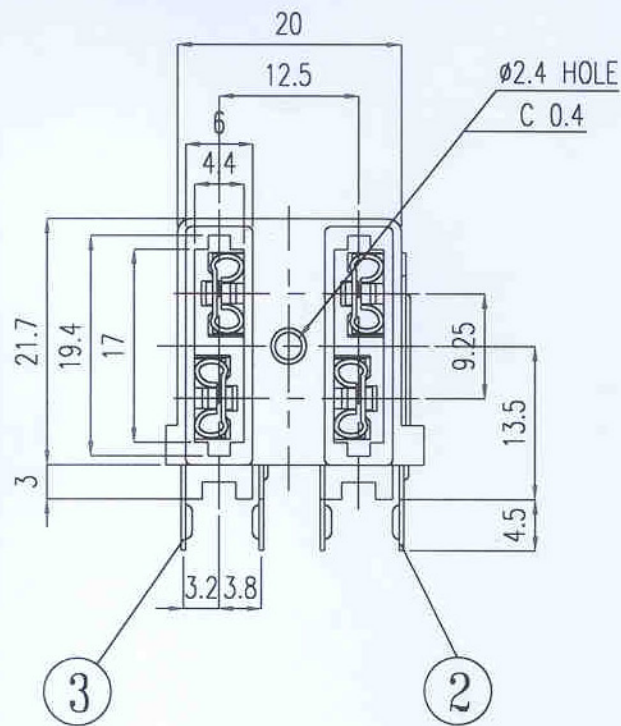
DETAIL "X"
