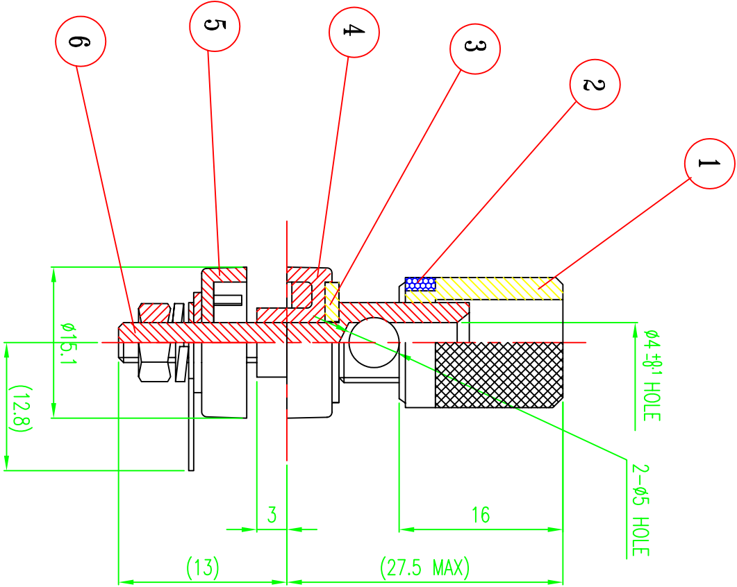
'A-A" SECTION
