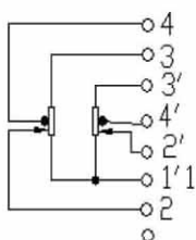
CIRCUIT
