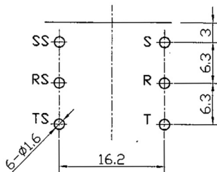
PCB MOUNTING HOLES (VIEWED FROM COPPER SIDE)
