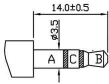
MATING PLUG
