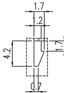
DETAIL "X" (2/1)
