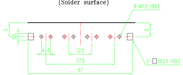
PCB-MTG (Solder surface)
