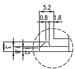
'C' DETAIL 2/1
